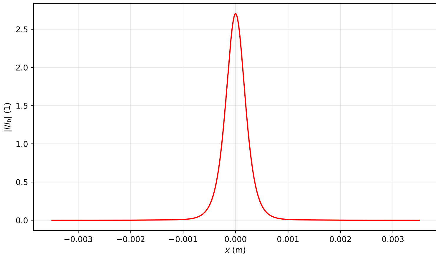
Intensity profile I(x, y = 0, z = 3.105)/I_0 , P_{in}=1.0P_{cr} , artificial time
